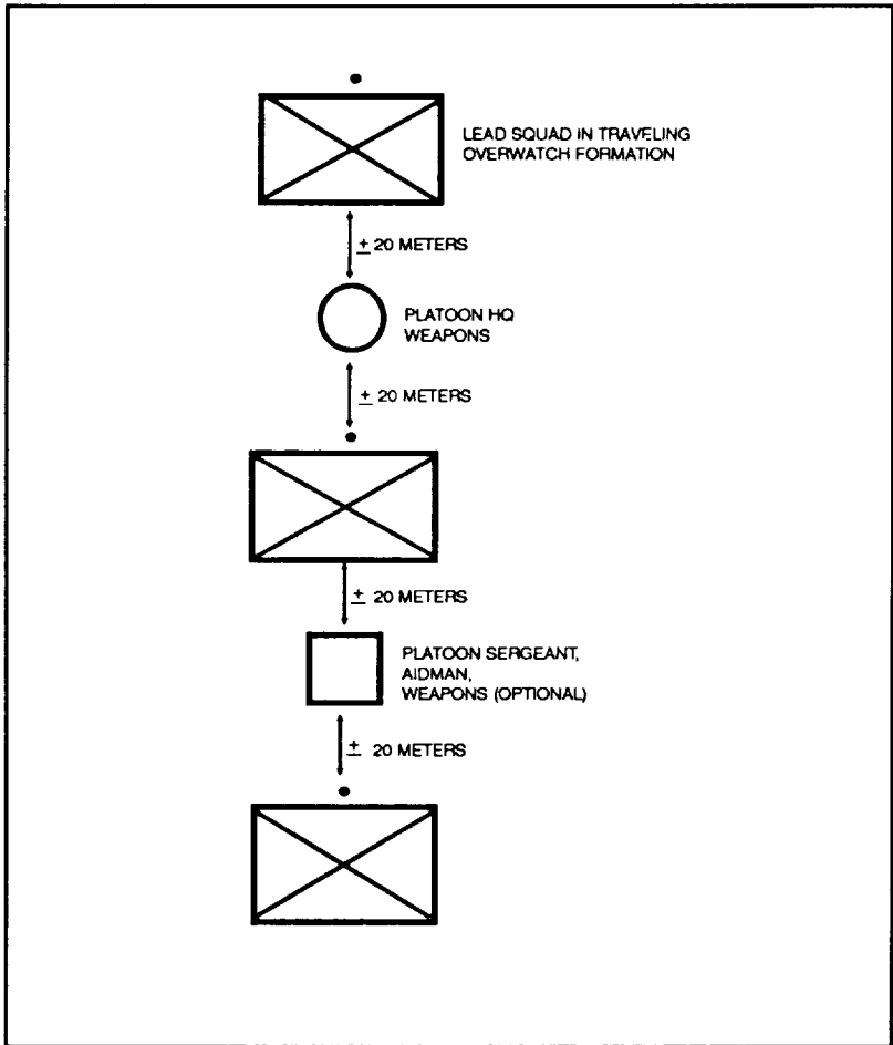
Figure 2-23. Platoon traveling.
